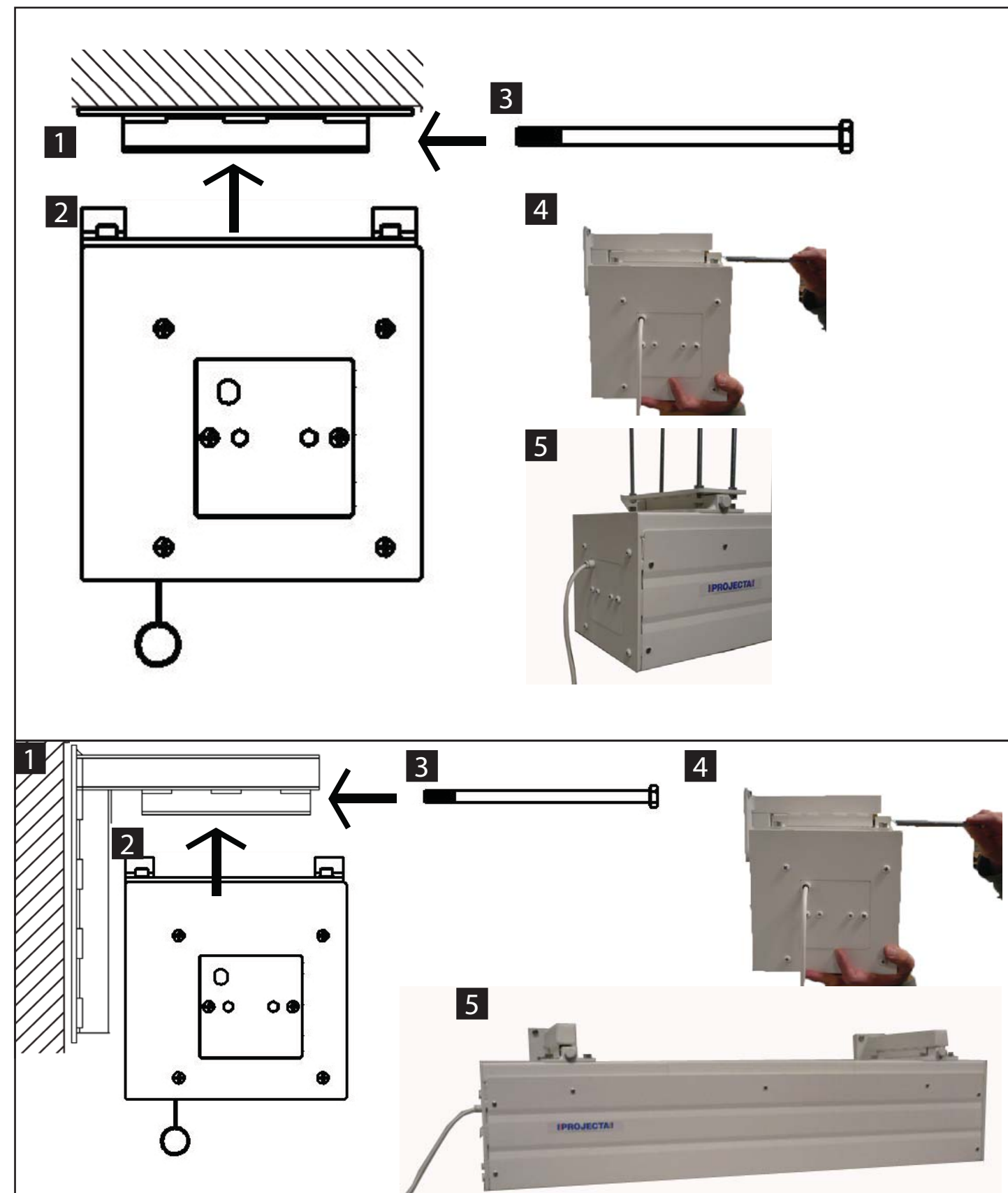
Mounting instruction
