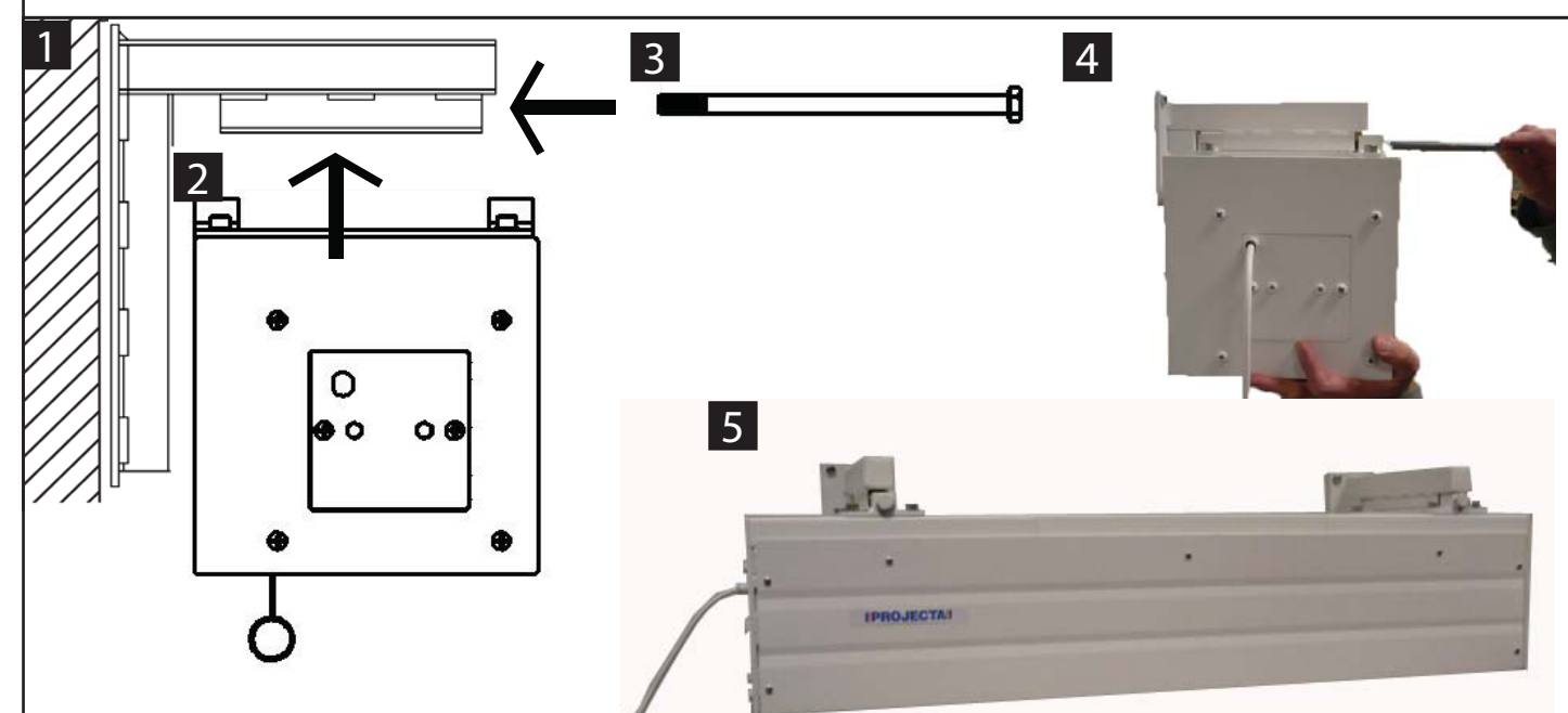
Mounting instruction
