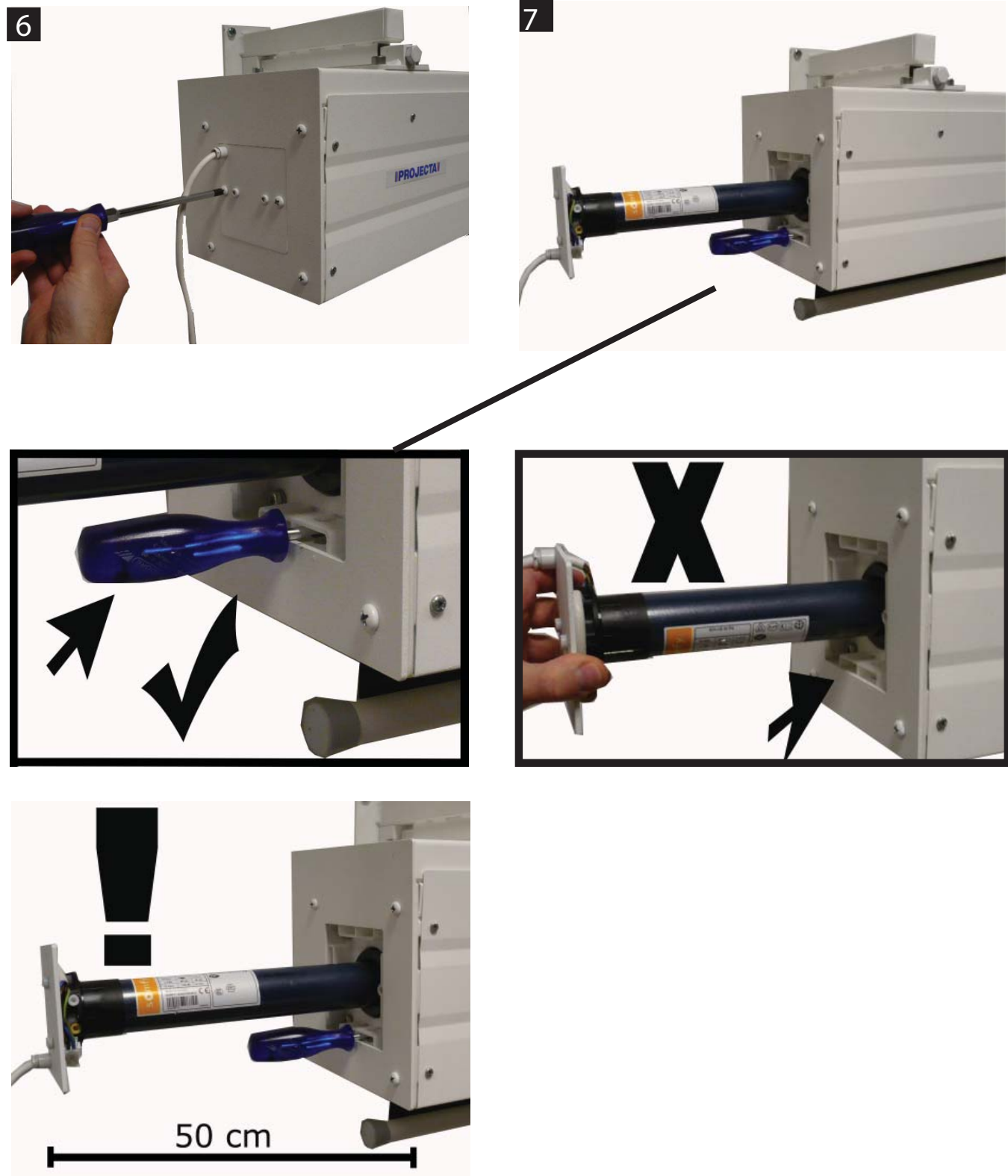
Mounting instruction
