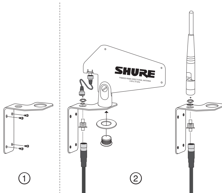
Wandmontage
